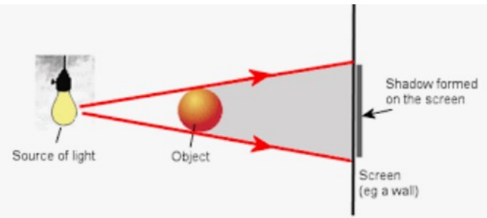
How a shadow is formed
