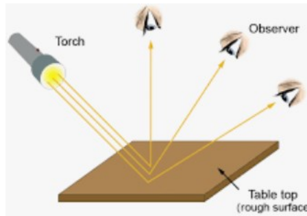
Light Reflecting off a surface
